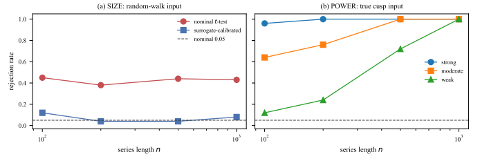
Fig. 2. (a) Size: on random-walk input the nominal t -test rejects at \approx 0.42 regardless of series length, while surrogate calibration restores approximately nominal size. (b) Power: of the calibrated test on input that genuinely contains a cusp. At the median observed length ( n \approx 200 ) strong and moderate dynamics are detected, weak dynamics largely are not.
